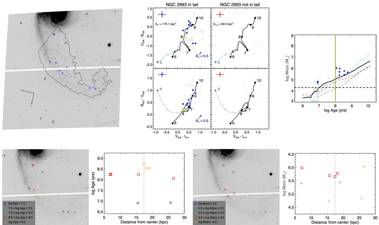
Figure 8. Same as 3, but for NGC 2993. We find 9 in-tail SCCs, and 0 out-of-tail SCCs. We capture the tidal tail of NGC 2993 (seen at the top of the image). Most of the SCCs in the tail have ages comparable to the interaction age of the NGC 2992/3 system.
