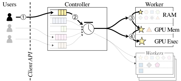
Fig. 3: Clockwork comprises multiple Workers and a centralized Controller. Models (★▲) reside on Workers; inference requests are queued and scheduled centrally on Clockwork’s Controller. See §4.1 for a detailed description.
