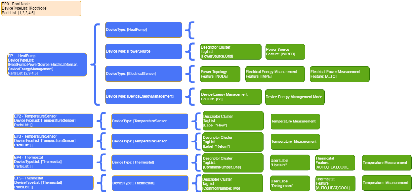
Figure 16. Example of a Heat Pump device
