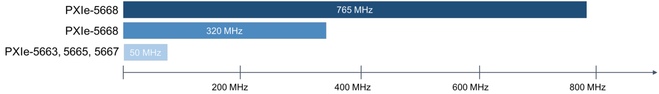
Figure 2. Available instantaneous RF bandwidth for NI VSAs
