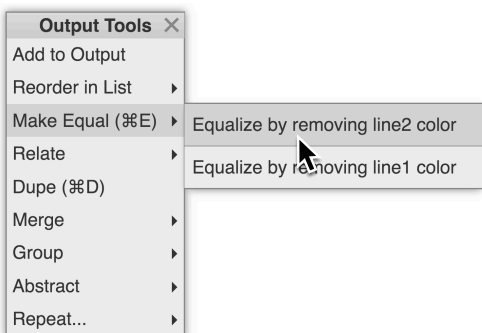
Figure 6. The output tools panel appears when an item on the canvas is selected. Each tool may offer multiple results; hovering the mouse over each result previews the change on the code and on the canvas.
